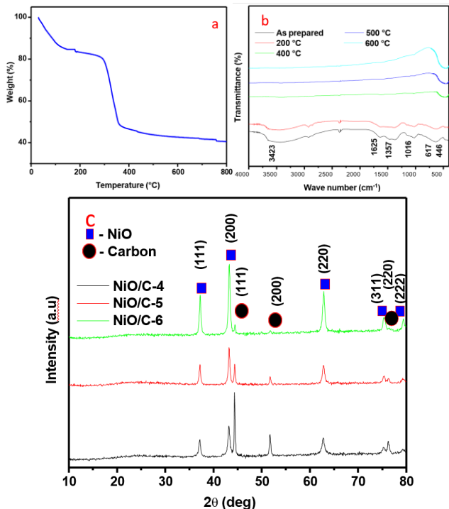
Fig. 1 a) TGA of uncalcined sample, b) FTIR spectrum of samples calcined at different temperatures and c) XRD pattern of NiO/C samples.
