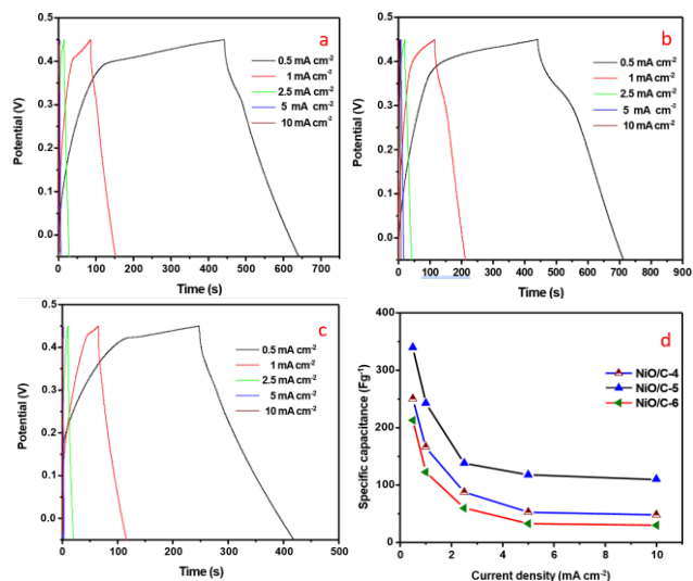
Fig. 6 Charge-discharge curves of (a) NiO/C-4, (b) NiO/C-5, and (c) NiO/C-6 electrodes at different current densities. (d) Variation of specific capacitance with current density.
